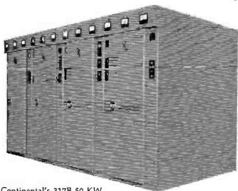
Continental's 317B 50 KW AM broadcast transmitter
